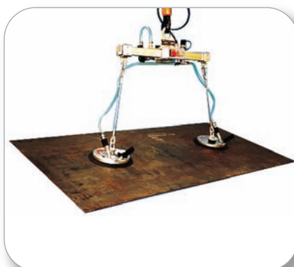
500 kg Horizontal Capacity
