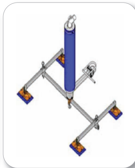
Large Panel - Suction Foot
