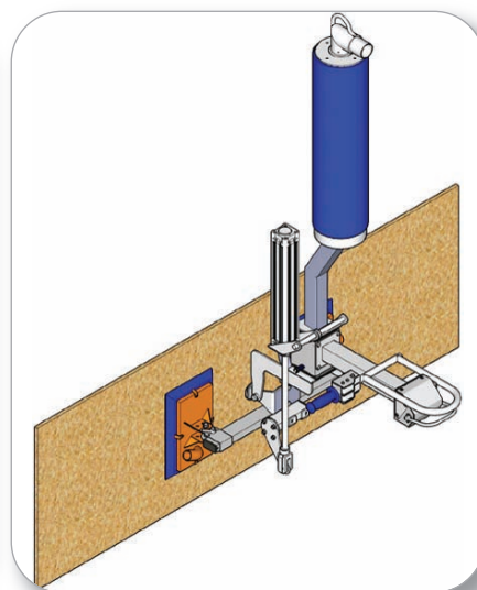
Powered 90° Turn
