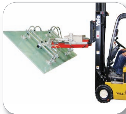
Truck Mounted Vacuum Gripper
